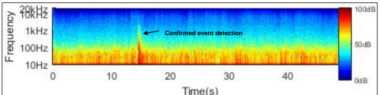
FIGURE 4.30: SPECTROGRAM – 20KG STATIC EVENT 11:26 13TH NOVEMBER 2014 – PEN_OS3
