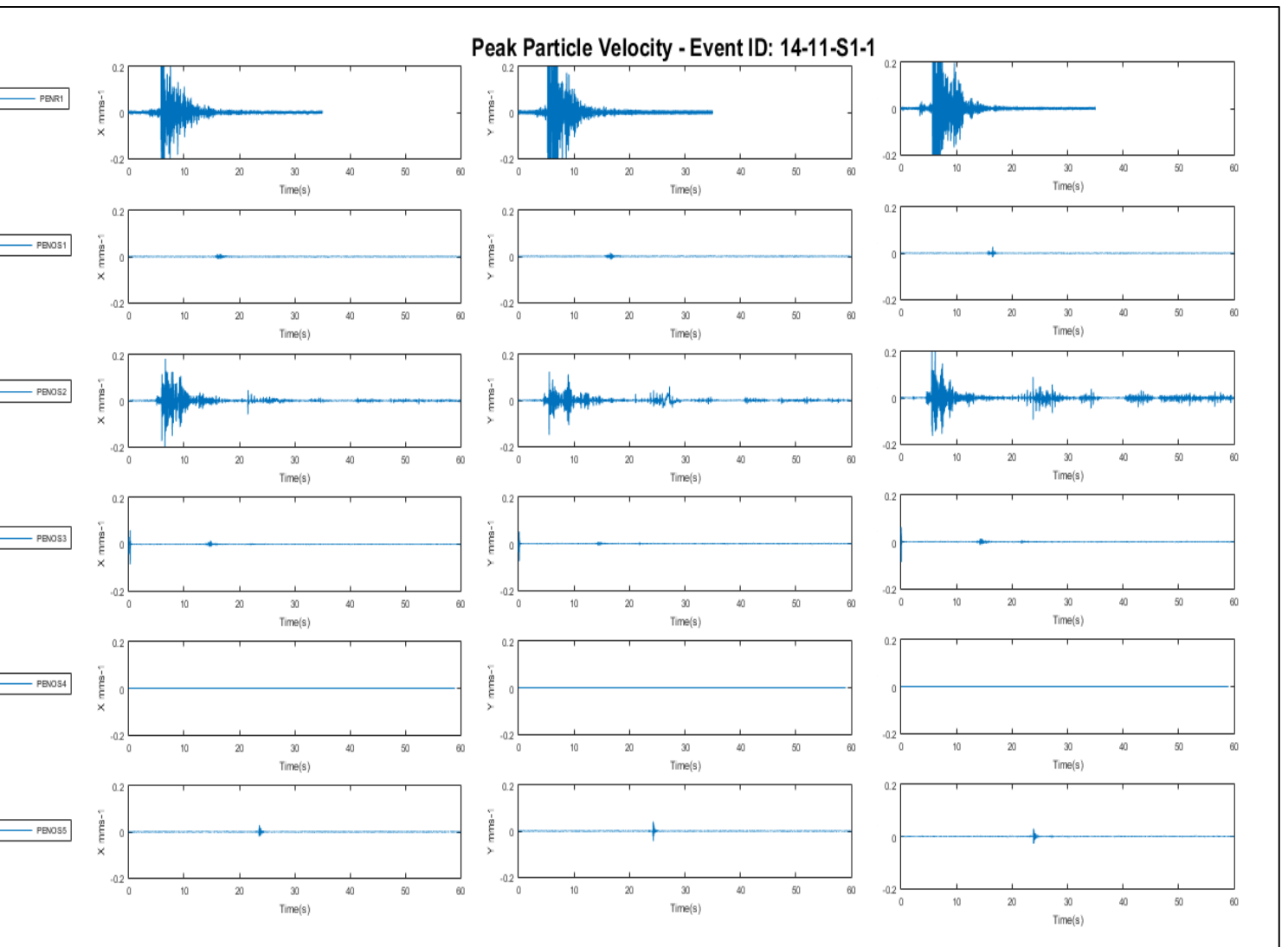
FIGURE 4.24: VELOCITY SIGNALS – 13KG DYNAMIC EVENT 14:48 24TH NOVEMBER 2014, PEN_OS1 – PEN_OS5
