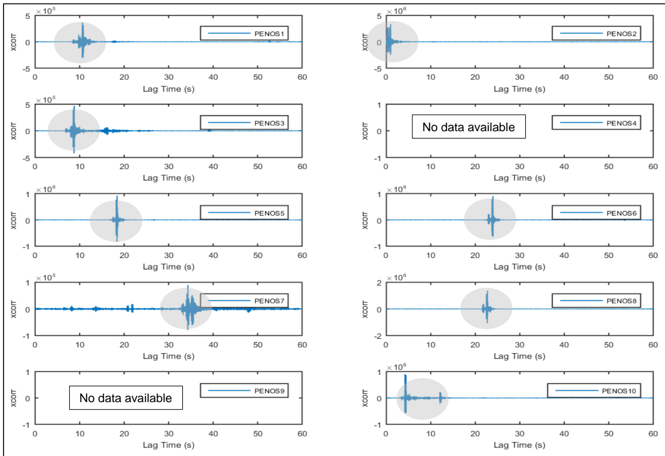
FIGURE 4.21: CROSS-CORRELATION – 13KG DYNAMIC EVENT 14:48 24TH NOVEMBER 2014
